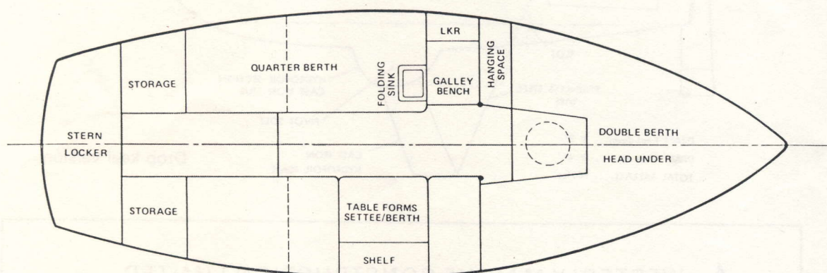
PLAN OF INTERIOR
