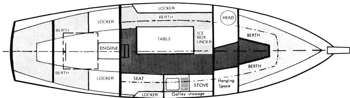
STOWAGE LOCKERS UNDER BERTHS
